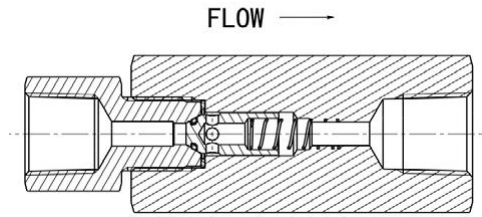
NPT 软密封单向阀
